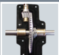
Fully Enclosed Metal Gears with Zerk Fittings
